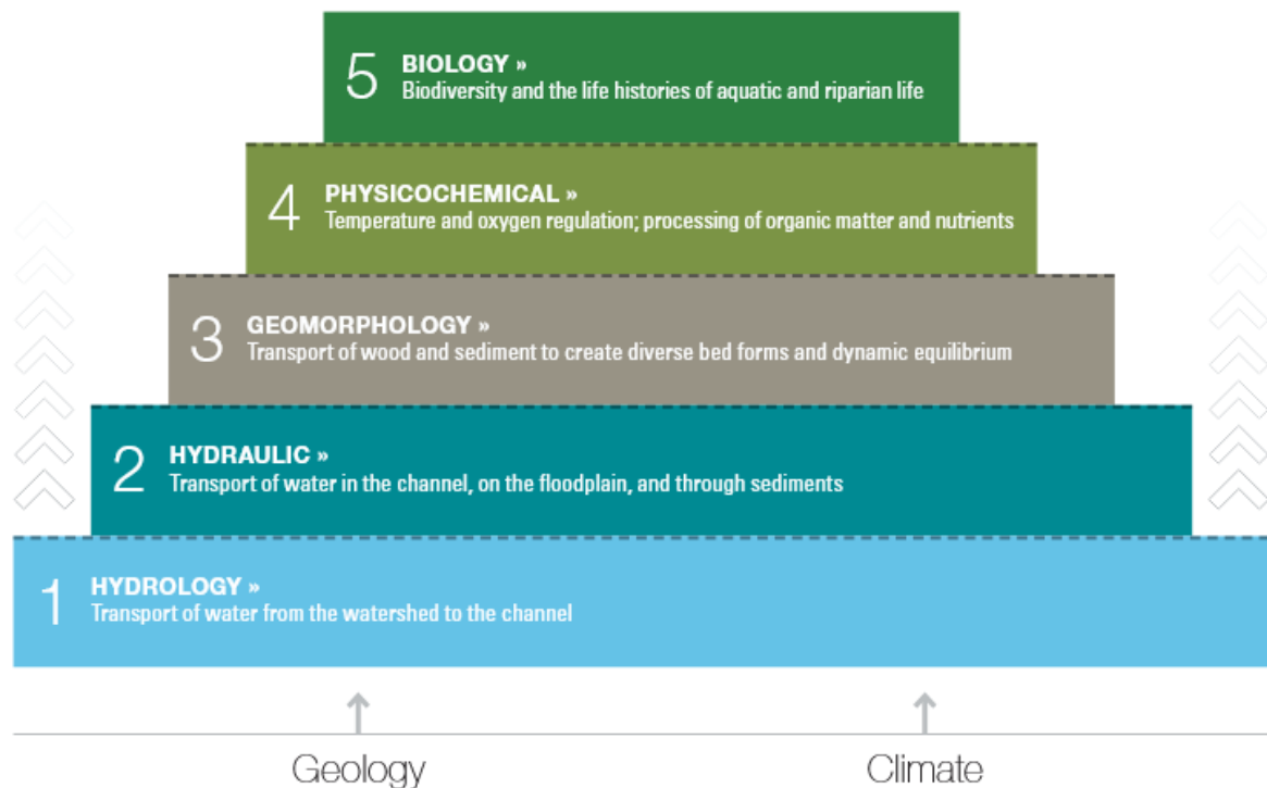
Figure 5: The Stream Functions Pyramid, developed by (Harman et al., 2012), provides a framework that organizes stream functions in a pyramid form. It illustrates that stream functions are supported by lower-level functions in a hierarchical structure.
