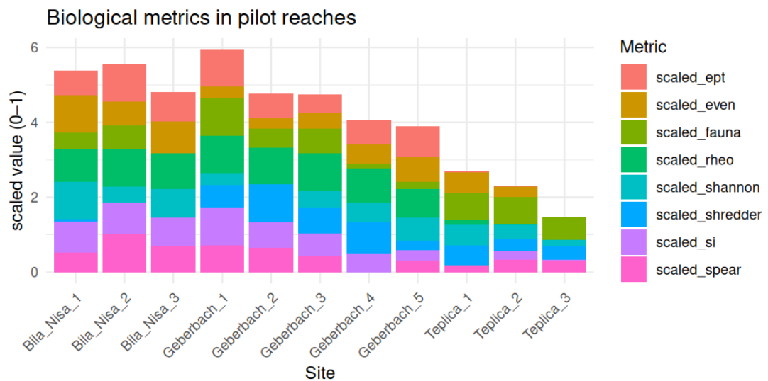
Figure 7: Selected normalized biological metrics in Teplica, Bila Nisa and Geberbach pilot sites, The first site of each stream is the urban reference site
