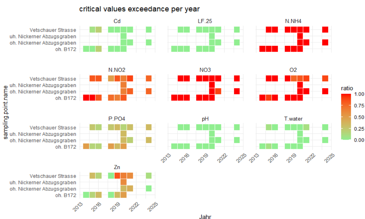
Figure 4 Exceedances of physico-chemical values per year (2013-2025) in different measurement stations in Geberbach. Red colour indicates a regular exceedance of ecocritical values, green colour indicates that no exceedance was measured. Data from Sächsischen Lan
