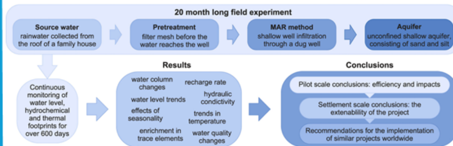
Conceptual scheme of rooftop rainwater harvesting using shallow well infiltration and groundwater recharge (Duna-Tisza Interfluvium, Hungary).
