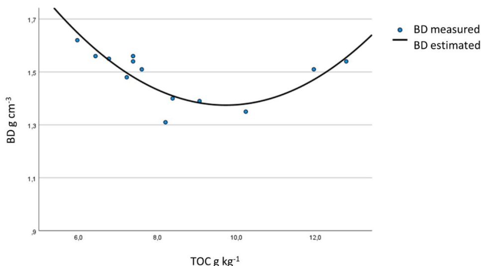
Figure 10: BD measured and BD predicted from TOC for the samples used PTF determination (N=13 out of 28).
