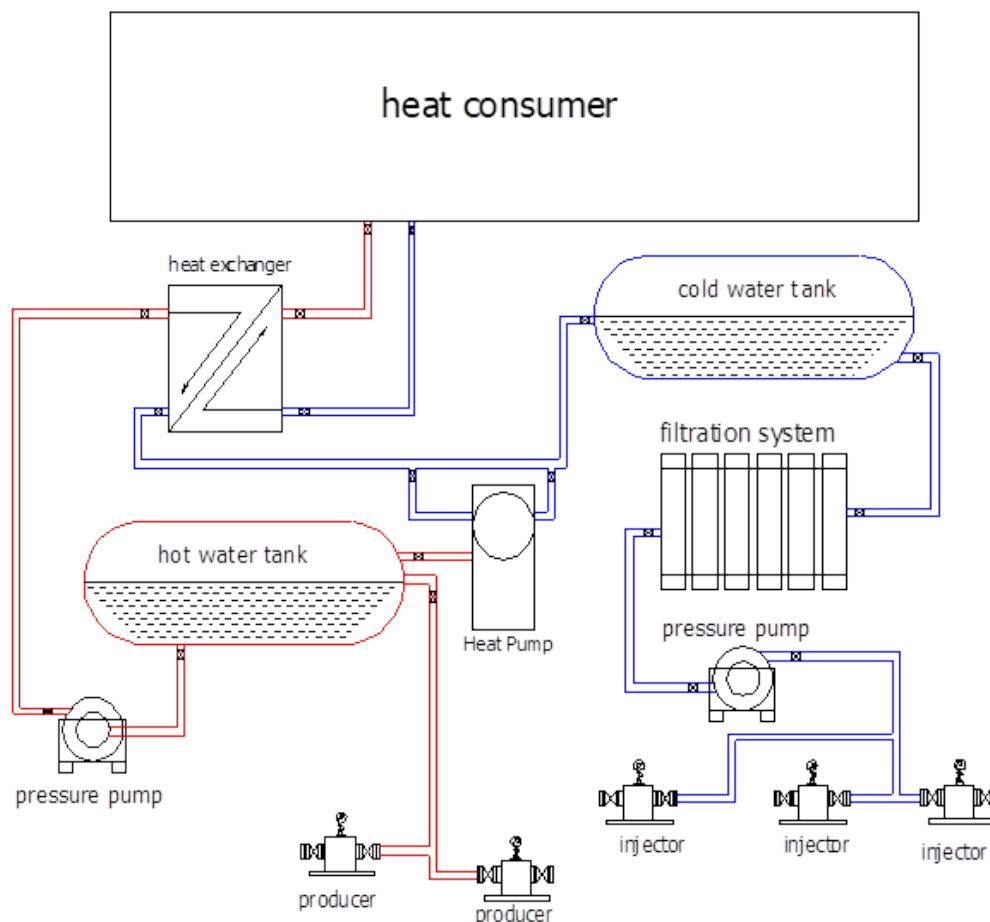
Figure 14. Typical surface equipment installation.
