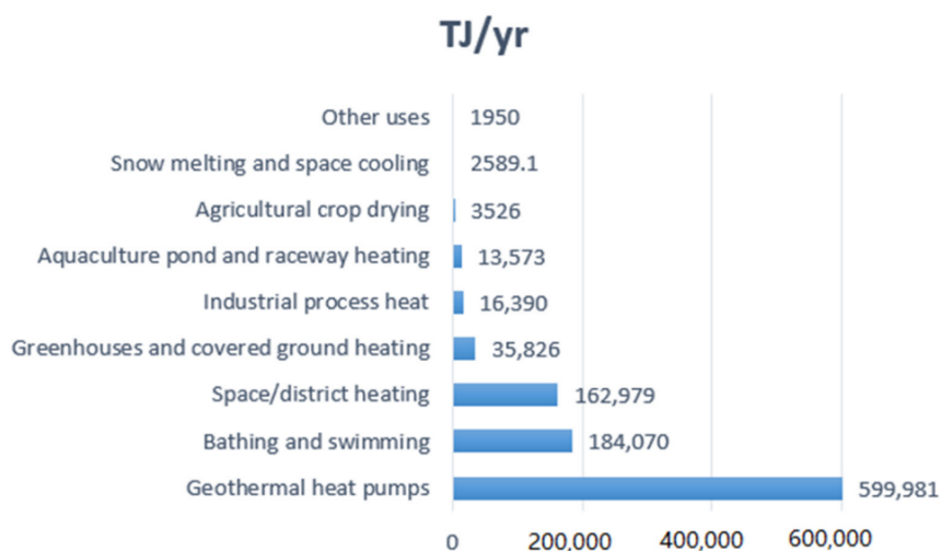
Figure 4. Worldwide direct use of geothermal energy in TJ/yr (Lund and Tot, 2021).
