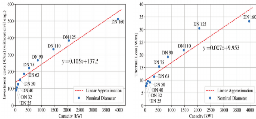
Figure 13. Correlation between investment cost versus capacity and thermal losses versus capacity (Röder et al., 2021).
