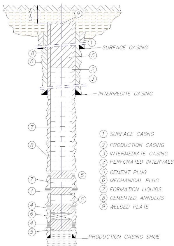
Figure 12. Typical application of an abandoned well.
