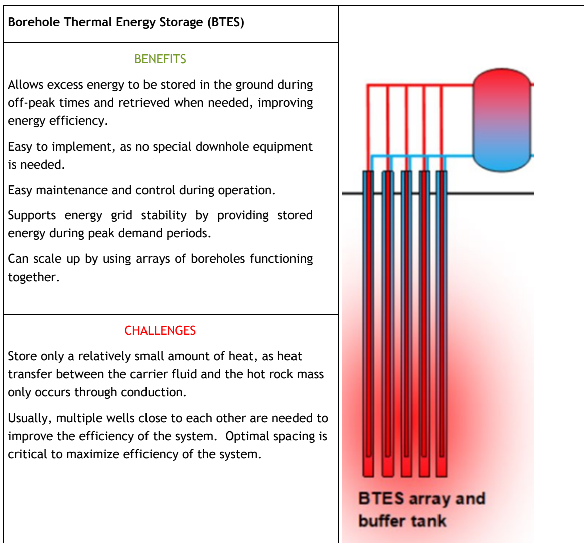
Figure 6. Borehole Thermal Energy Storage (BTES) (Kolo et al., 2024).
