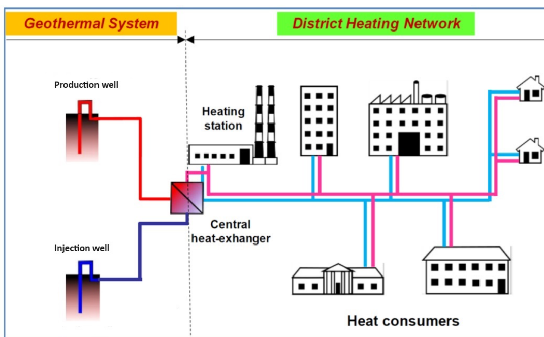
Figure 2. District heating system application with a geothermal system (adapted from Barkaoui et al., 2018).
