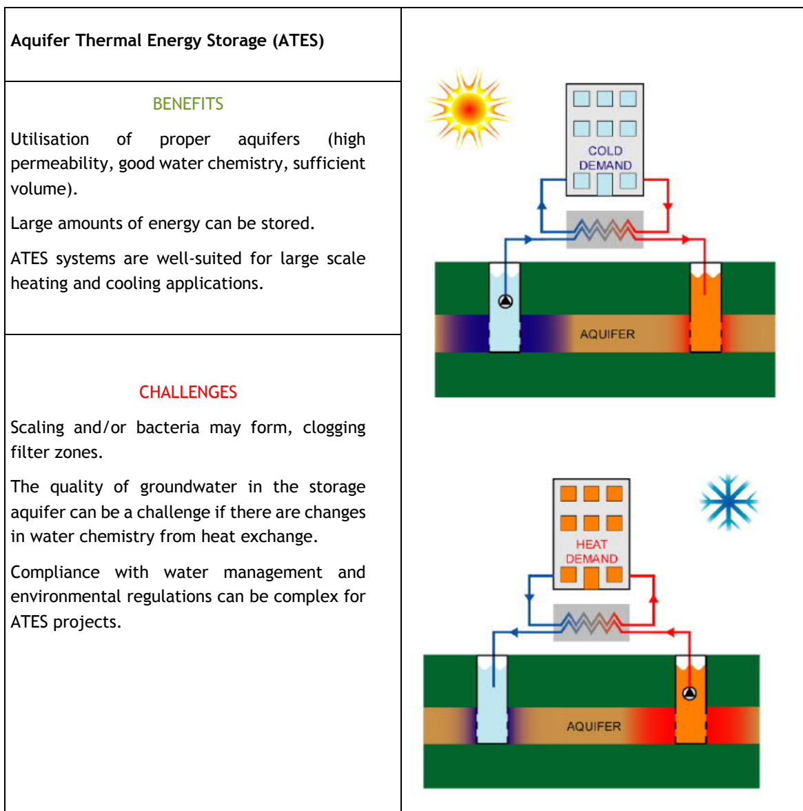
Figure 7. Aquifer Thermal Energy Storage (ATES) (Drijver et al., 2003).
