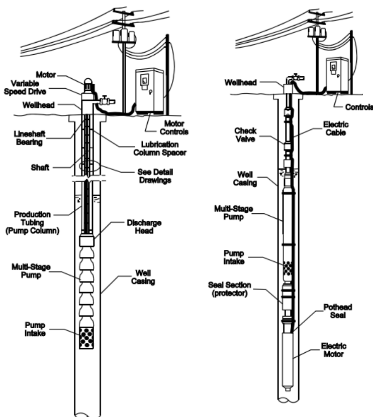
Figure 15. Downhole pump systems: line shaft pump (left) and electrical submersible pump (right) (Lund, 1998).
