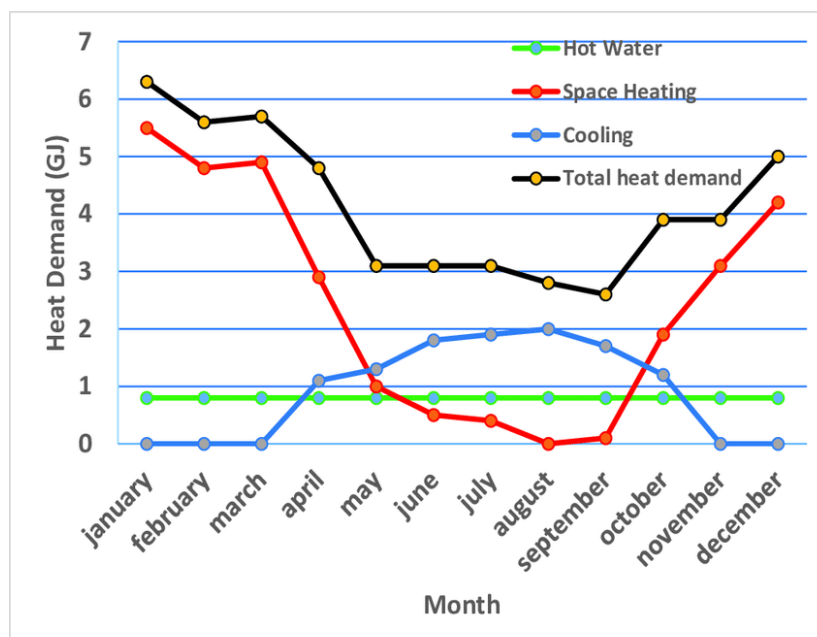
Figure 1. Typical heating demand over a year in a district heating system (Geusa et al., 2014).
