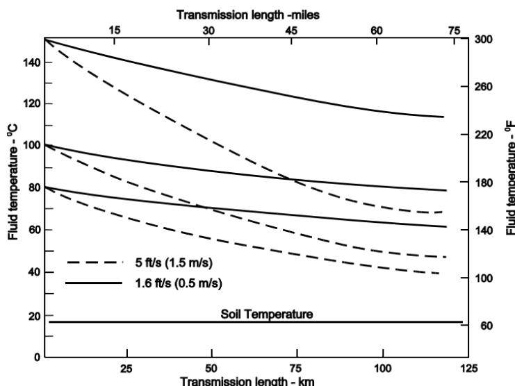
Figure 16. Temperature drop in a hot-water transmission line (Lund, 1998).
