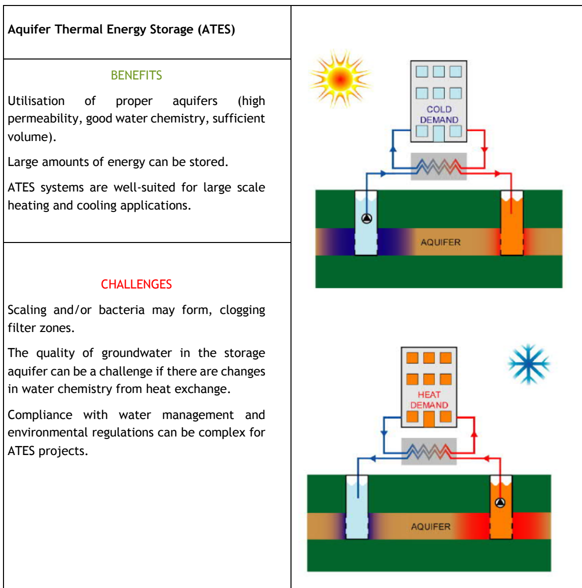
Figure 11. Aquifer Thermal Energy Storage (ATES) (Drijver et al., 2003).
