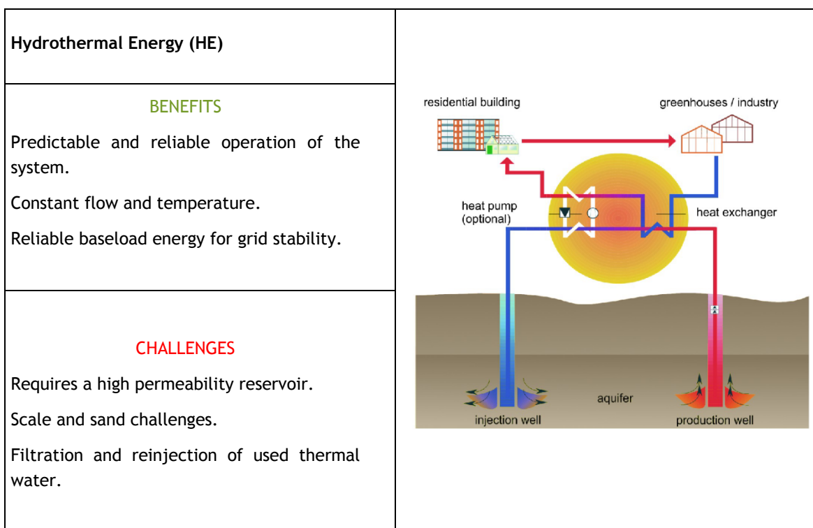
Figure 12. Hydrothermal Energy (HE) (Agemar et al., 2014).
