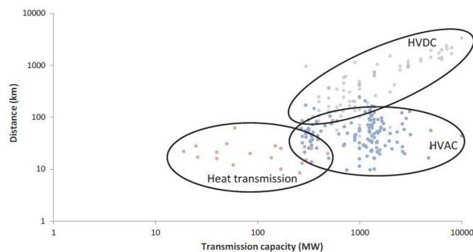
Fig. 1. Comparison of energy transmission different energy carriers.
