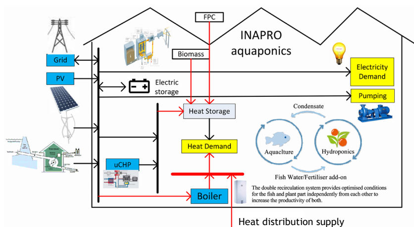
Figure 7. Hybrid energy system for aquaculture/aquaponics (adapted from Karimanzira, 2018).
