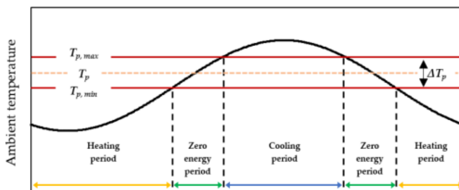
Figure 4. Conceptual greenhouse demand pattern over one year (Dimitropoulou et al., 2023).
