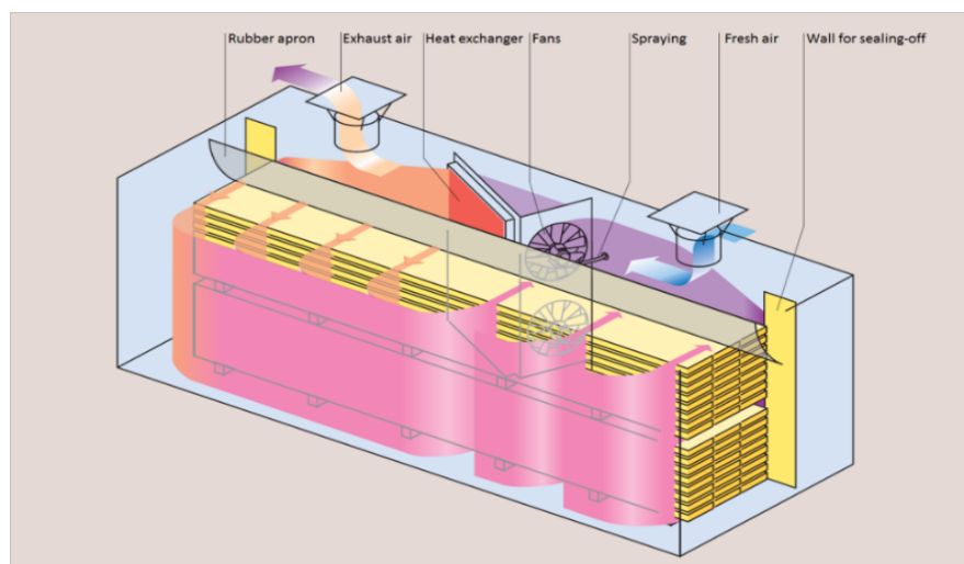
Figure 6. Transverse ventilation system for wood drying (Lauber Holzrockner, 2024).
