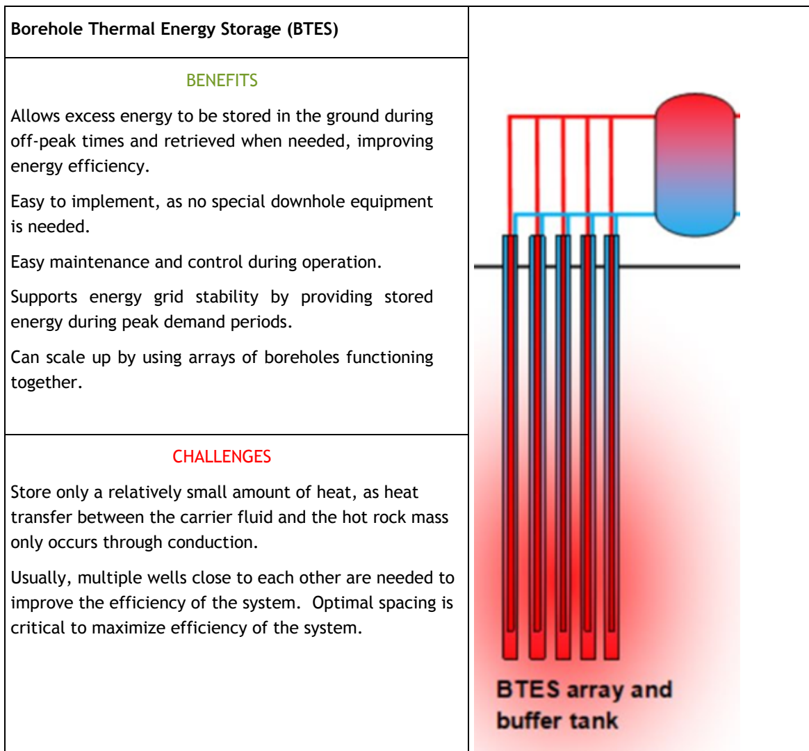
Figure 10. Borehole Thermal Energy Storage (BTES) (Kolo et al., 2024).
