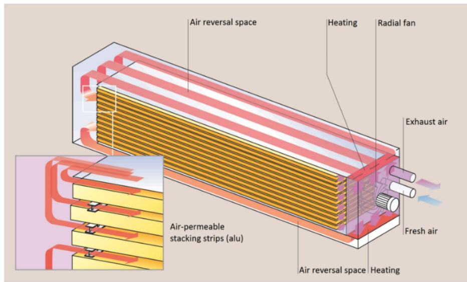
Figure 5. Longitudinal ventilation system for wood drying (Lauber Holzrockner, 2024).
