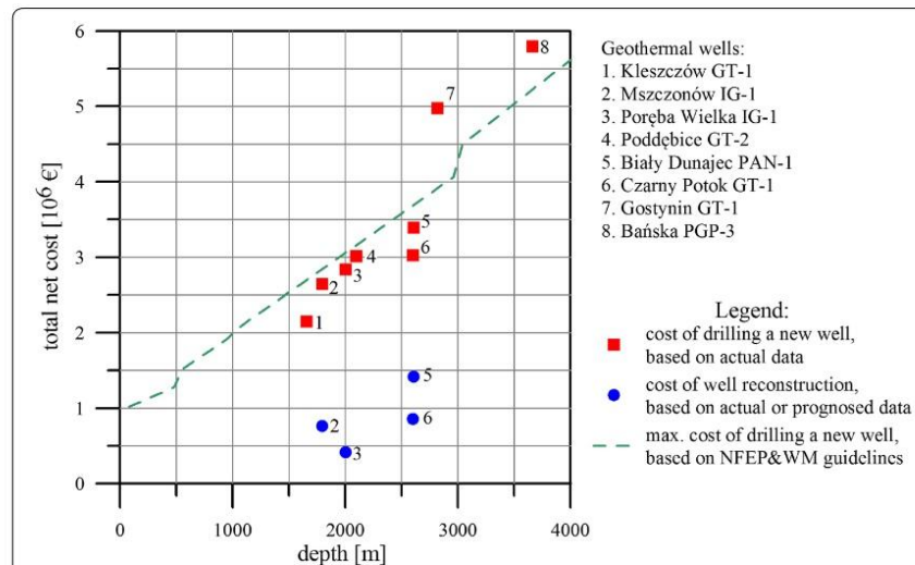
Fig. 16 A summary of the actual costs of drilling and reconstructing selected geothermal wells in Poland
