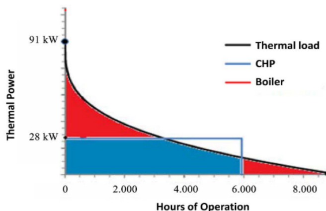
Figure 8. Annual heat load curve for an aquaculture/aquaponics system of 360 m 2 floor area (Karimanzira, 2018).
