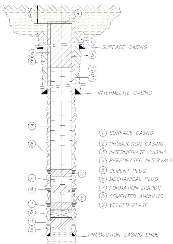
Figure 15. Typical application of an abandoned well.
