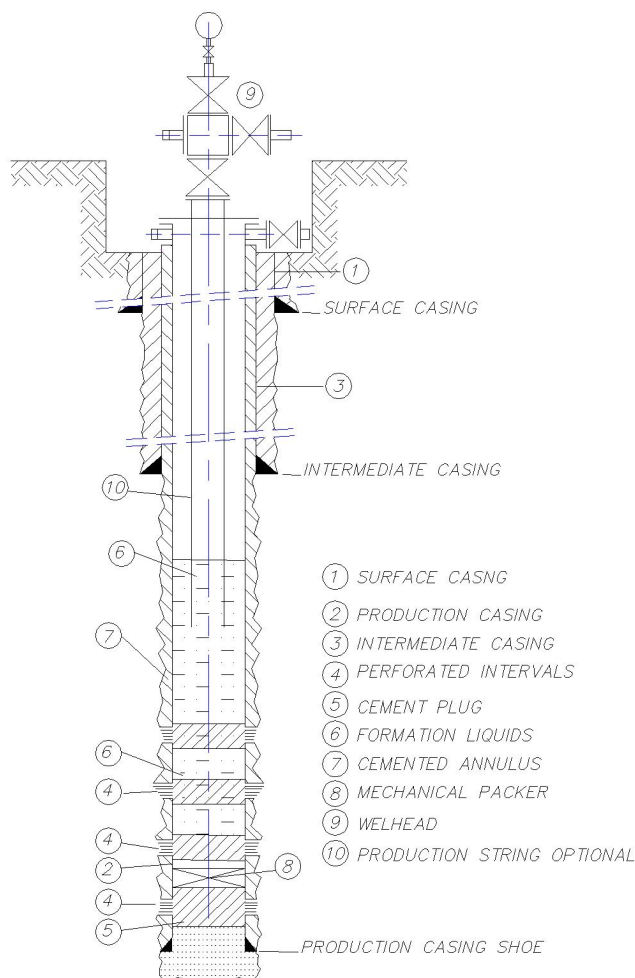
Figure 14. Typical configuration of a shut-in well.
