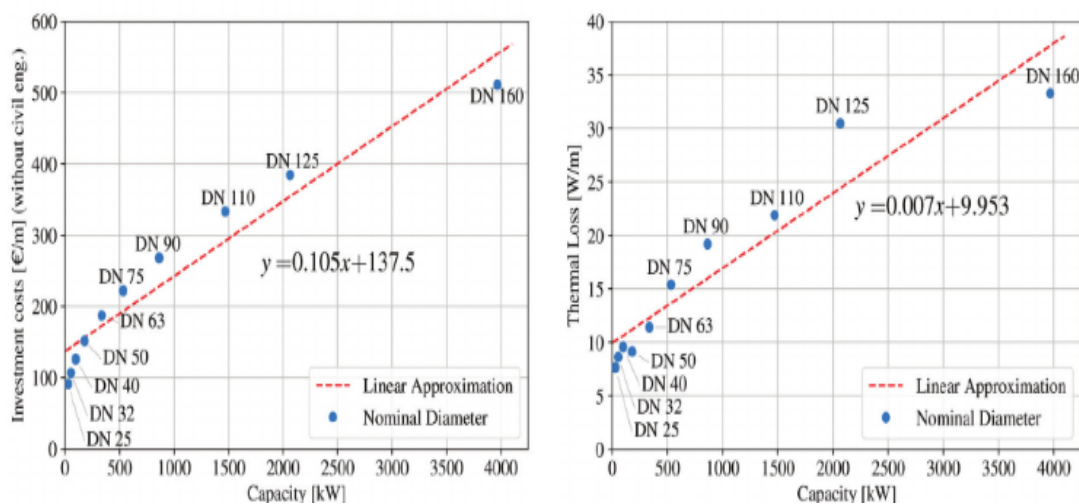
Figure 16. Correlation between investment cost versus capacity and thermal losses versus capacity (Röder et al., 2021).
