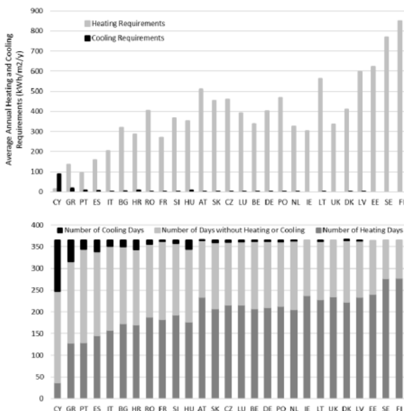
Figure 1. Summary of heating and cooling demand of greenhouses in EU countries (Tataraki et al., 2020).
